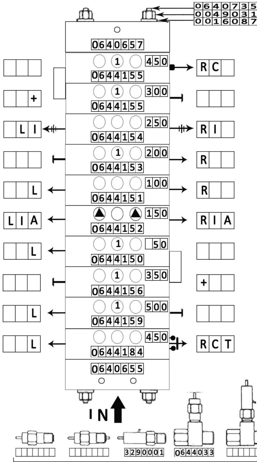
CONNECTION ELEMENT
